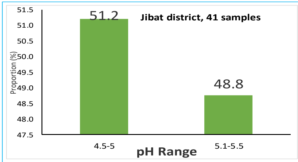
Fig.2 Distribution of soil acidity in Jibat and Ifata District of the study site based on soil exchangeable acidity and pH of collected soil sample
