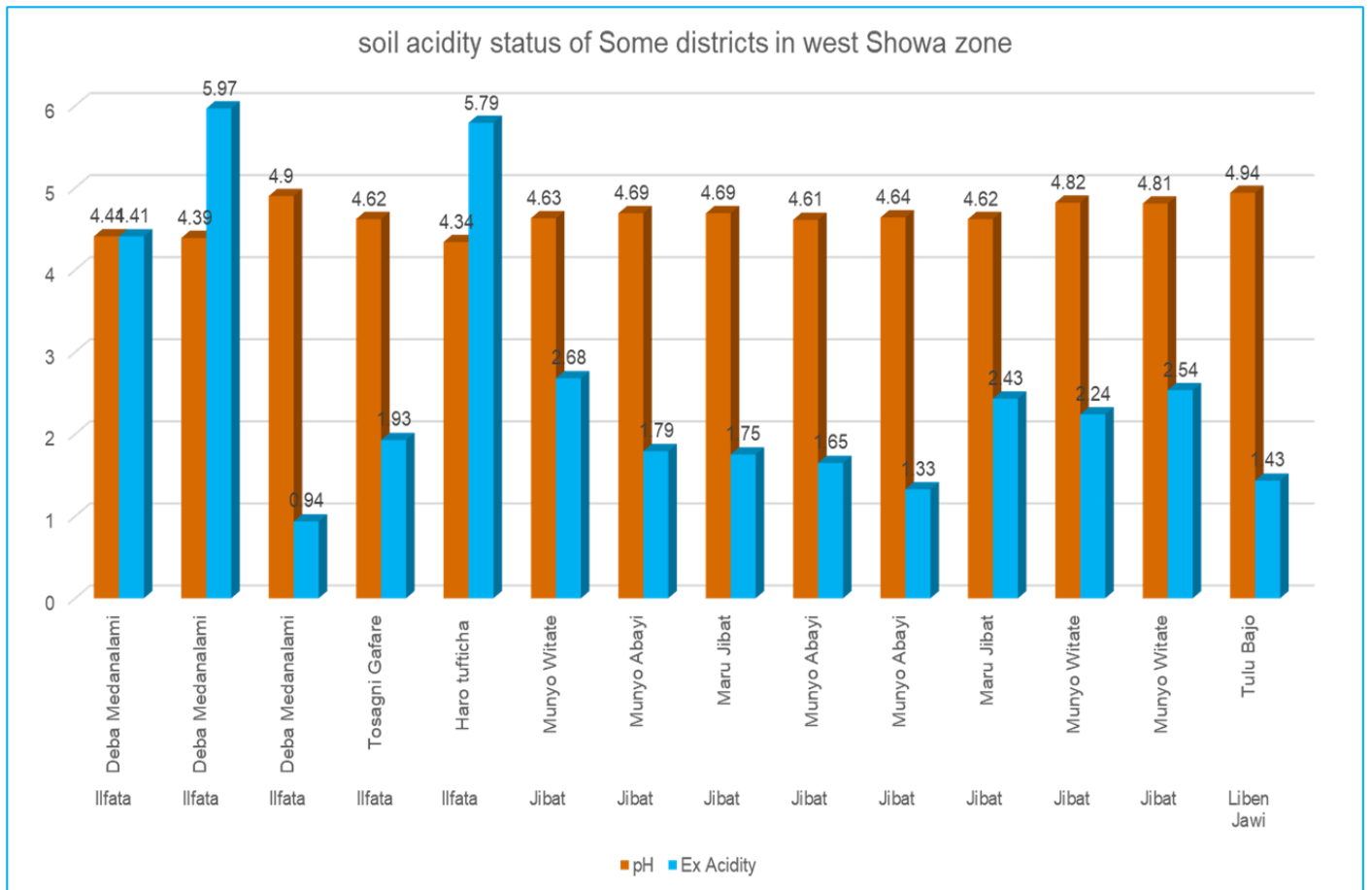
Fig.2 Distribution of soil acidity in Jibat and Ifata District of the study site based on soil exchangeable acidity and pH of collected soil sample
